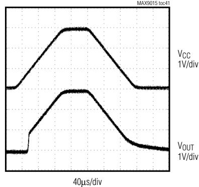
SLOW POWER-UP/DOWN RESPONSE MAX9015 toc41
